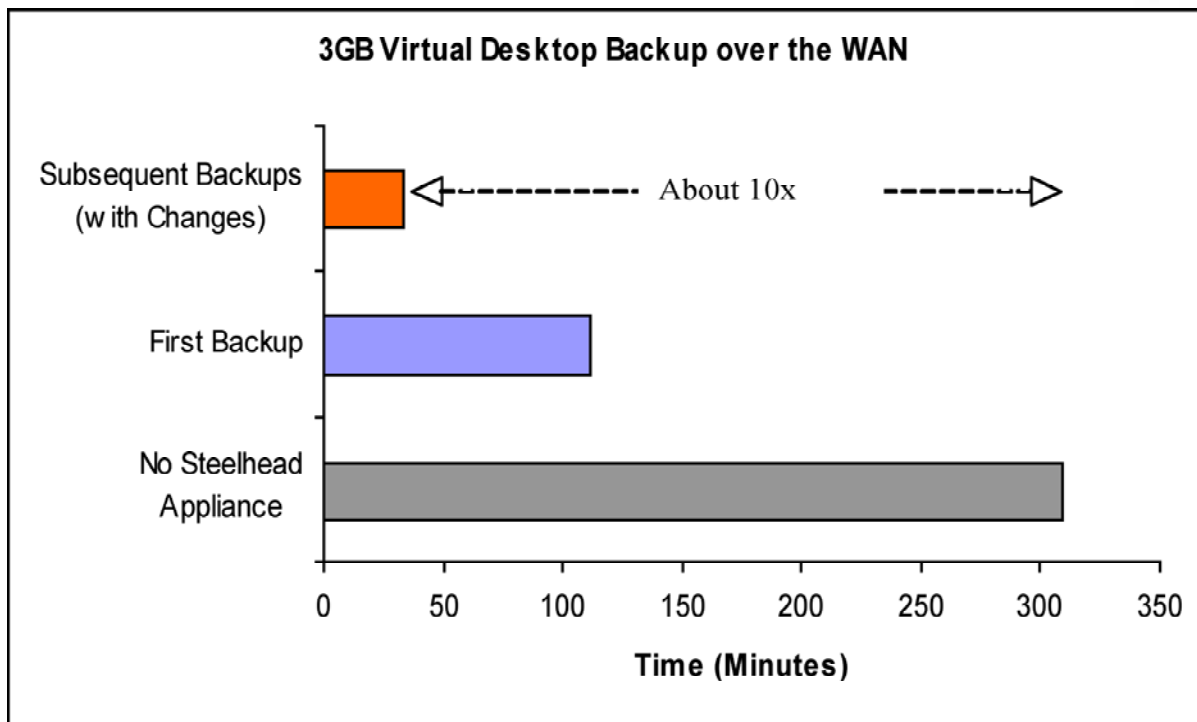
Chart 2. Backup of desktop images over a T1 with 100ms latency using WAN optimization solutions can be accelerated dramatically. This compliments a local desktop virtualization gateway by enabling all desktop images to be stored centrally, yet still accessed locally.
