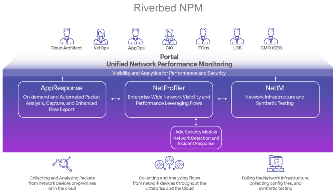
Figure 7: Riverbed unified NPM integrates packet data from AppResponse, flow data from NetProfiler, infrastructure polling from NetIM and security monitoring from NetProfiler Advanced Security Module and brings all the data together into unified, role-based views in Portal.
