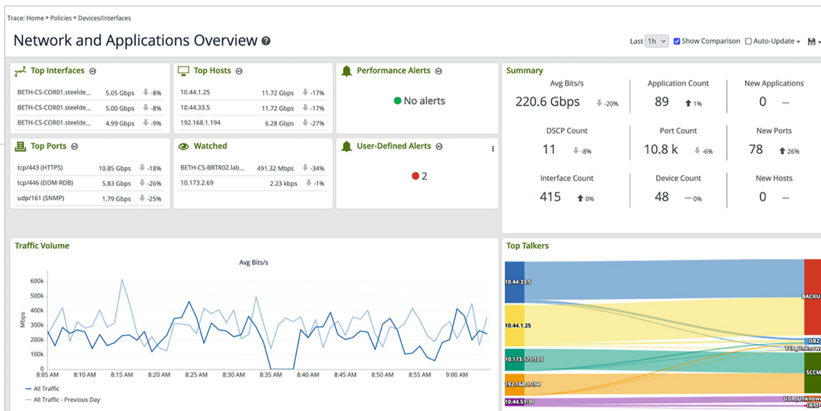
Figure 1: Personalizable to each user, the NetProfiler Home Screen offers an at-a-glance summary of the network and how it's changed; recent alerts; Top Talkers Sankey; overall traffic charts, and a watch list so you can see what's important to you.
