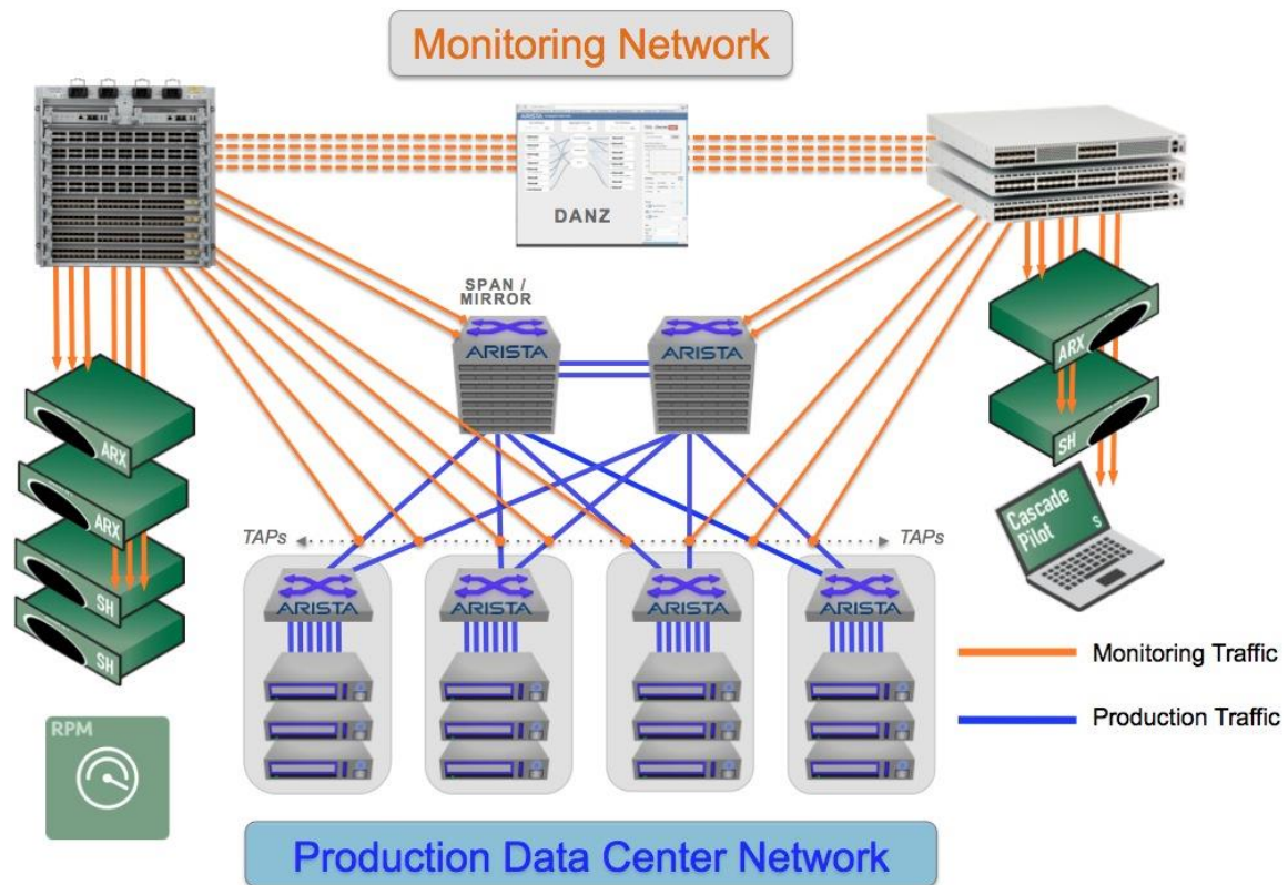
Figure 1. Arista Switches with DANZ, shown as both infrastructure with advanced port-mirroring (a.k.a., SPAN) enabled at spine layer, and TAP aggregation mode enabled in dedicated monitoring switches for scalable traffic capture, conditioning and load balancing of visibility traffic in a large cloud-scale data center network.
